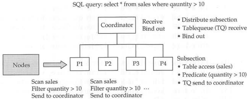
Figure 28.14 DB2 MPP query processing using function shipping.
