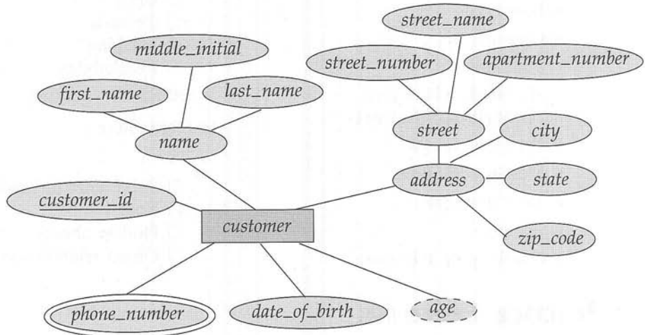
Figure 9.5 E-R diagram with composite, multivalued, and derived attributes.
