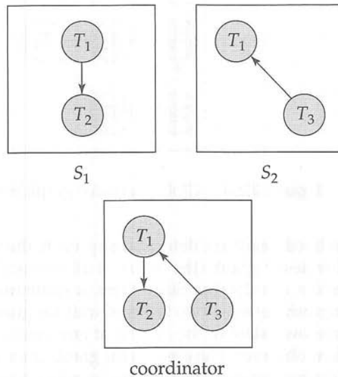
Figure 22.5 False cycles in the global wait-for graph.
