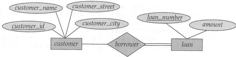
Figure 6.13 Total participation of an entity set in a relationship set.
