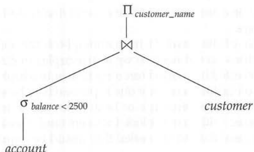
Figure 13.10 Pictorial representation of an expression.
