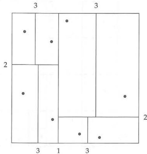
Figure 24.4 Division of space by a k-d tree.
