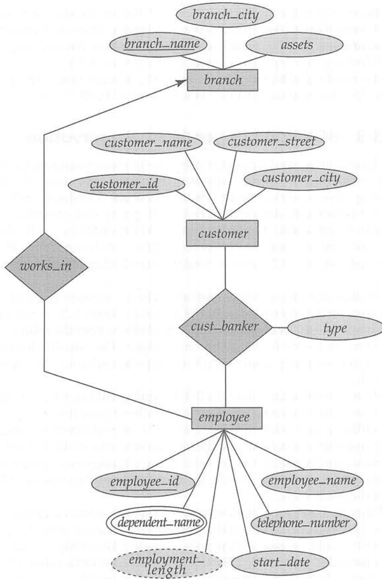
Figure 7.6 The cust_banker and works_in relationship sets.
