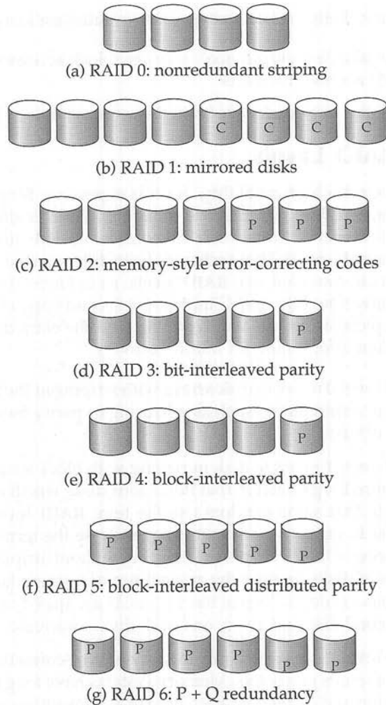
Figure 11.3 RAID levels.
