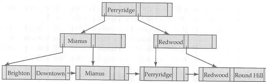
Figure 12.8 B + -tree for account file ( n = 3 ).
