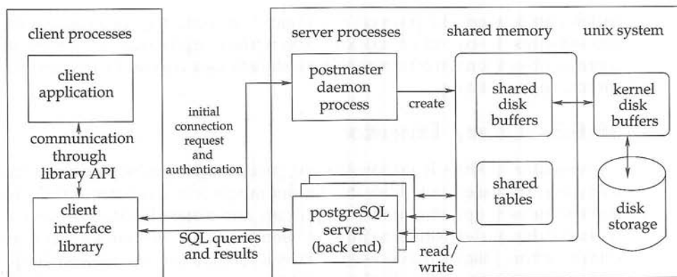
Figure 26.9 The PostgreSQL system architecture.
