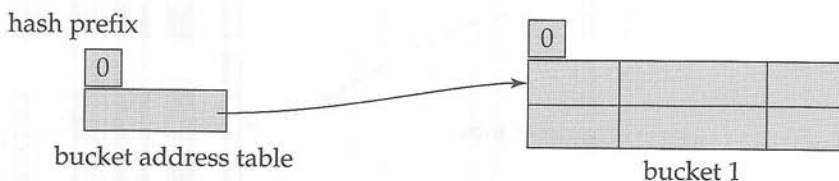
Figure 12.27 Initial extendable hash structure.
