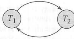
Figure 15.16 Precedence graph for schedule 4.
