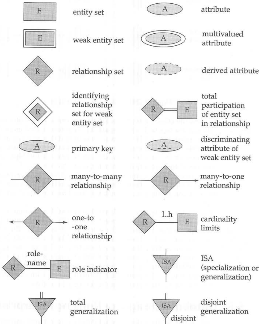
Figure 6.23 Symbols used in the E-R notation.
