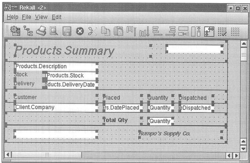
Figure 26.4 Rekall: Report-design GUI.
