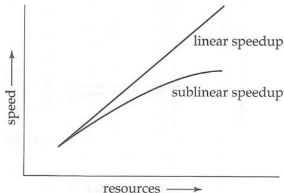
Figure 20.5 Speedup with increasing resources.
