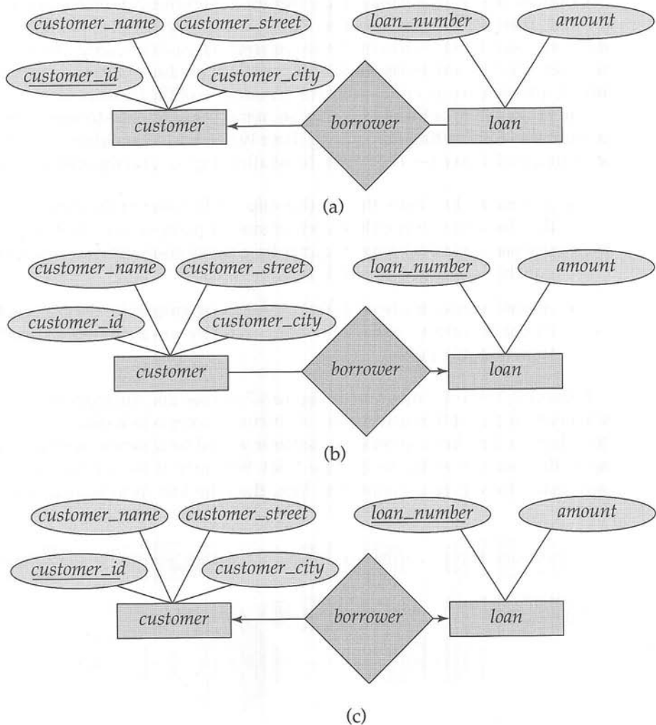
Figure 6.8 Relationships. (a) One-to-many. (b) Many-to-one. (c) One-to-one.
