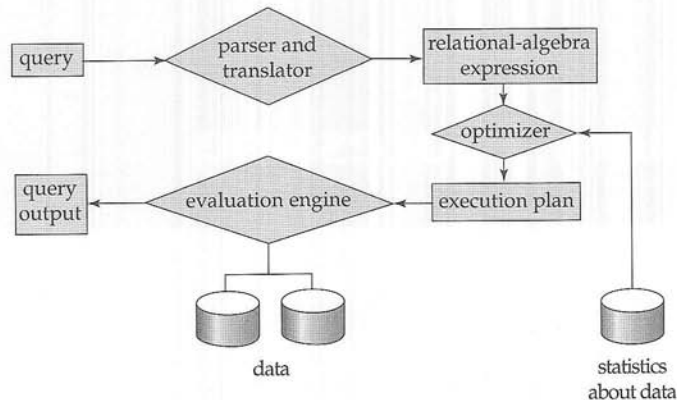
Figure 13.1 Steps in query processing.
