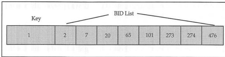
(b) Dimension block index entry for item Id = 1
