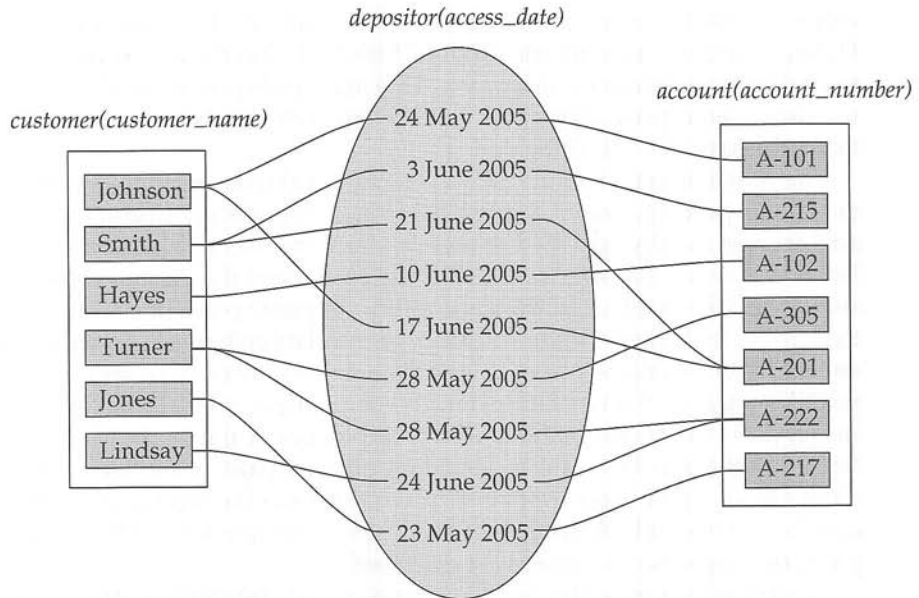
Figure 6.3 Access_date as attribute of the depositor relationship set.
