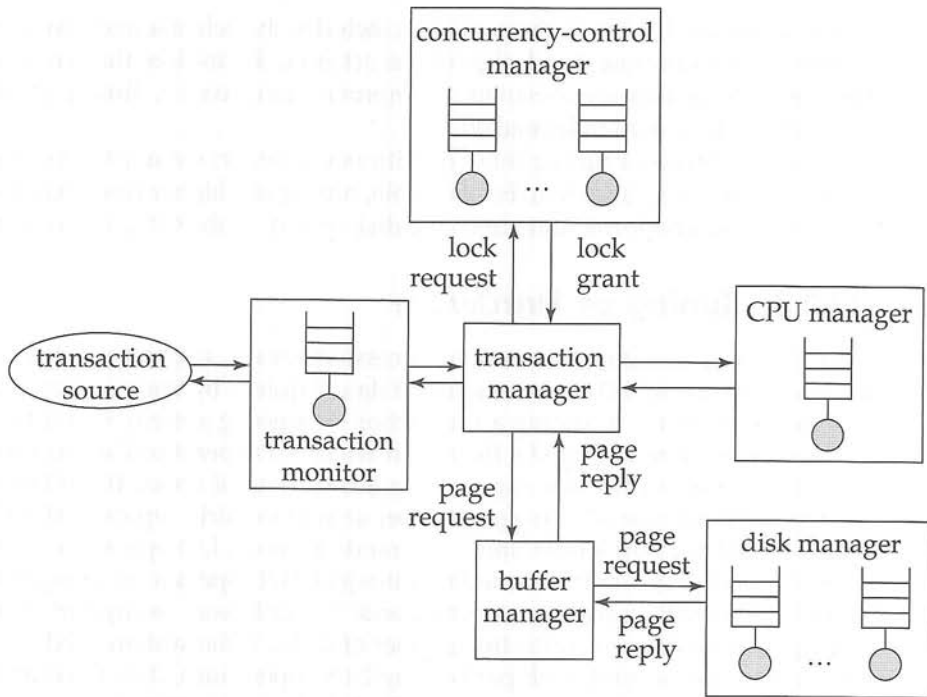
Figure 23.1 Queues in a database system.
