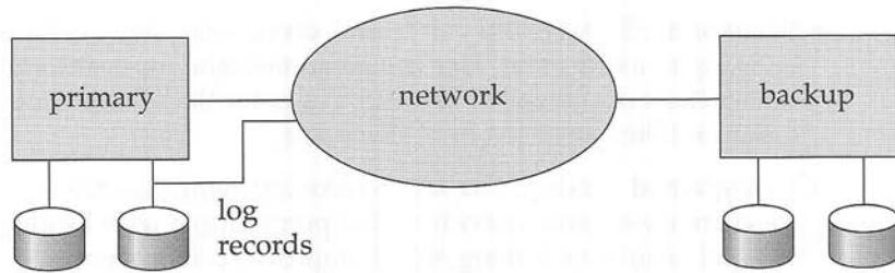
Figure 17.8 Architecture of remote backup system.
