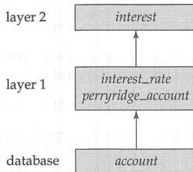
Figure 5.10 Layering of view relations.
