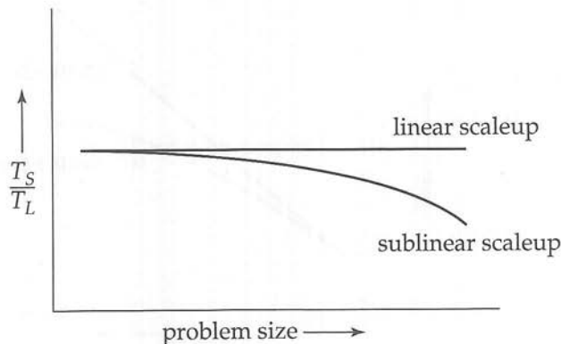
Figure 20.6 Scaleup with increasing problem size and resources.
