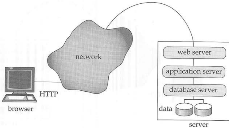
Figure 8.4 Three-layer Web architecture.
