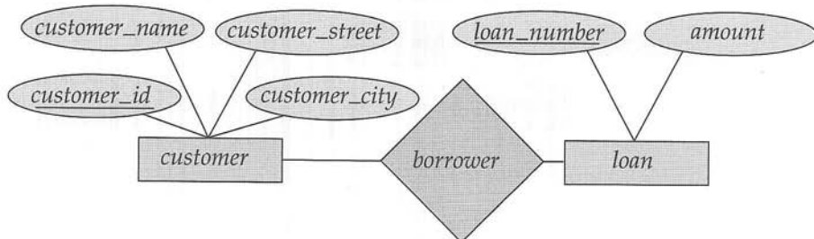
Figure 6.7 E-R diagram corresponding to customers and loans.
