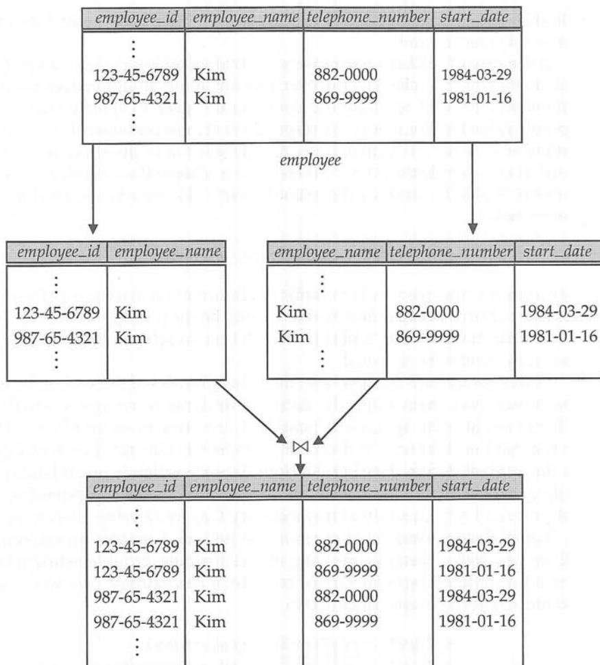
Figure 7.4 Loss of information via a bad decomposition.
