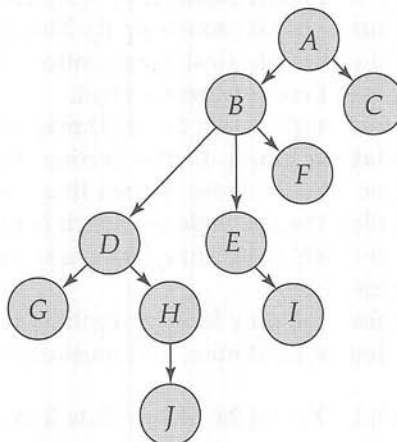
Figure 16.11 Tree-structured database graph.
