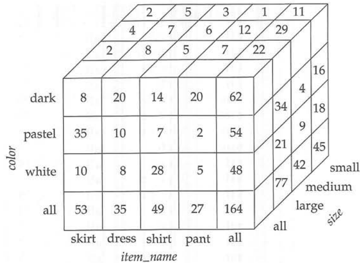
Figure 18.3 Three-dimensional data cube.
