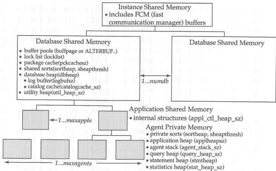
Figure 28.21 DB2 memory model.
