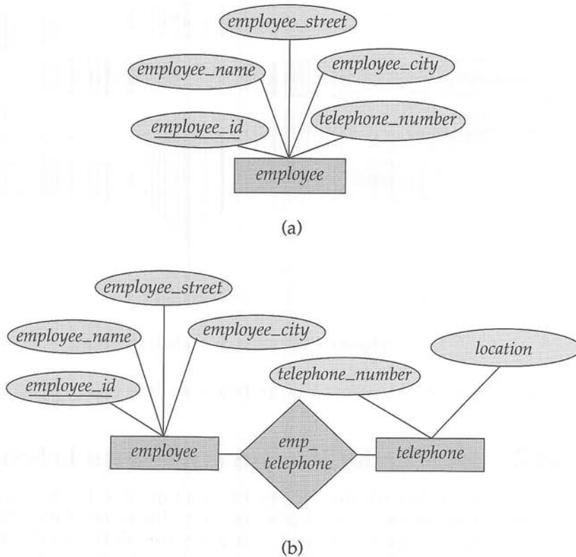
Figure 6.15 Alternatives for employee and telephone .
