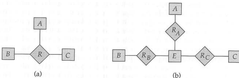
Figure 6.17 Ternary relationship versus three binary relationships.
