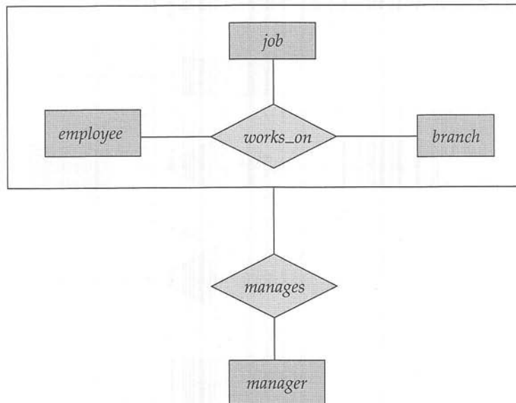
Figure 6.22 E-R diagram with aggregation.
