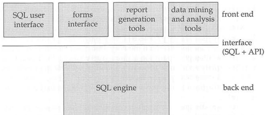
Figure 20.3 Front-end and back-end functionality.
