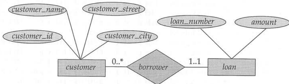
Figure 6.14 Cardinality limits on relationship sets.
