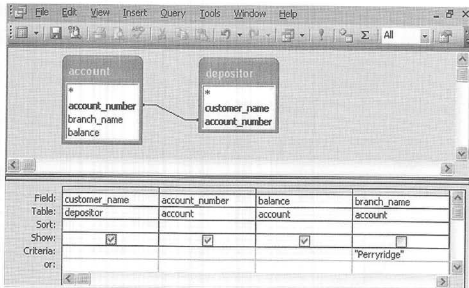
Figure 5.3 An example query in Microsoft Access QBE.
