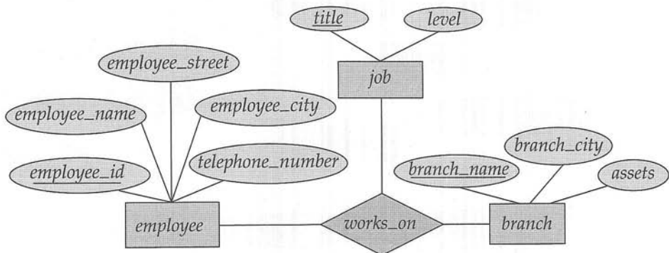
Figure 6.12 E-R diagram with a ternary relationship.
