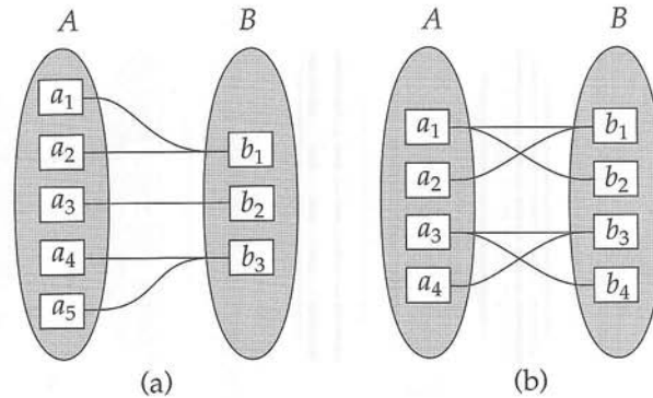
Figure 6.6 Mapping cardinalities. (a) Many-to-one. (b) Many-to-many.
