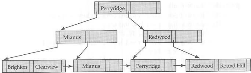
Figure 12.14 Deletion of “Downtown” from the B + -tree of Figure 12.12.
