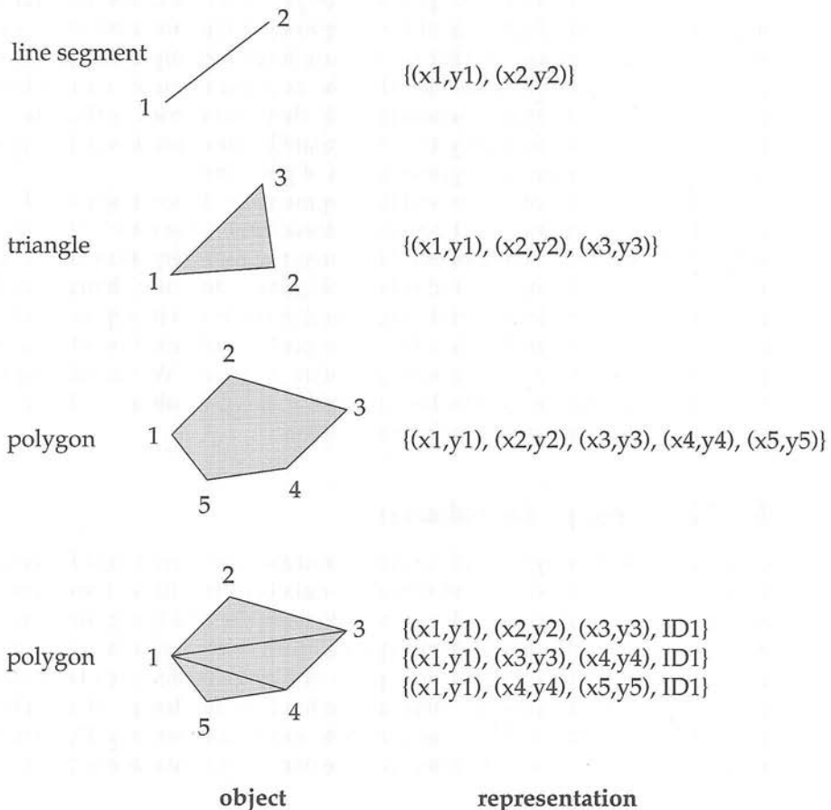
Figure 24.2 Representation of geometric constructs.
