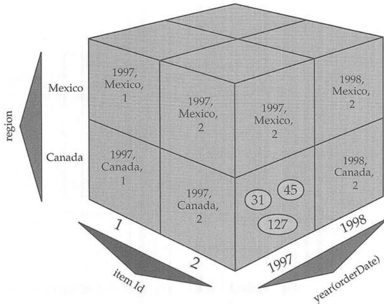
Figure 28.9 Logical view of physical layout of an MDC table.
