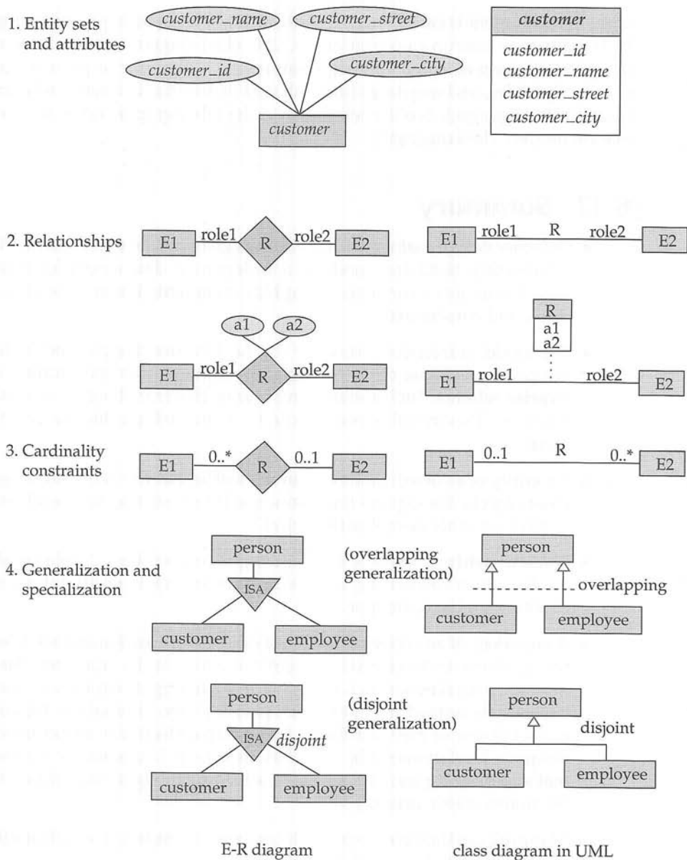
Figure 6.28 Symbols used in the UML class diagram notation.
