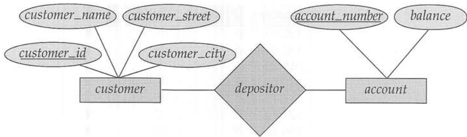
Figure 1.3 A sample E-R diagram.
