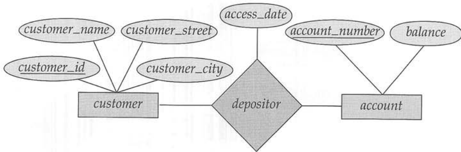
Figure 6.9 E-R diagram with an attribute attached to a relationship set.
