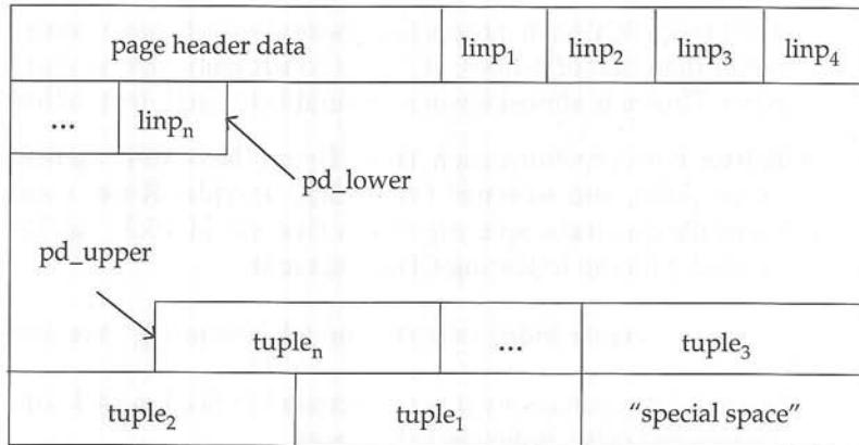
Figure 26.8 Slotted-page format for PostgreSQL tables.
