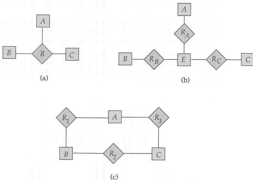
Figure 6.29 E-R diagram for Practice Exercise 6.9 and Exercise 6.22.
