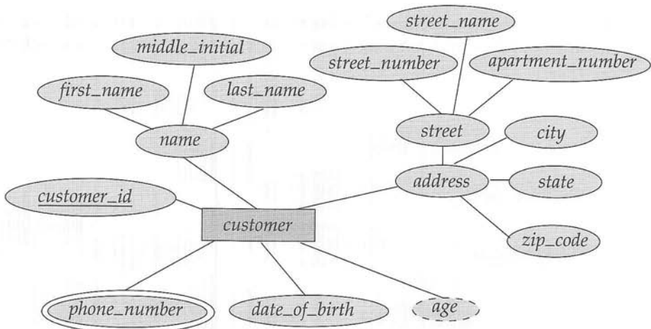
Figure 6.10 E-R diagram with composite, multivalued, and derived attributes.
