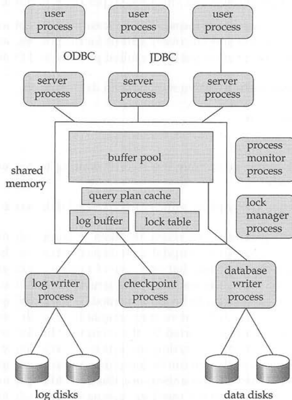
Figure 20.4 Shared memory and process structure.
