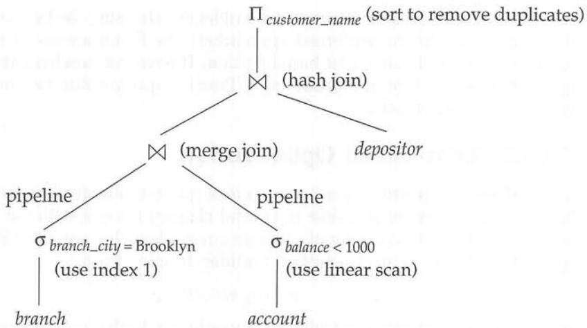
Figure 14.5 An evaluation plan.
