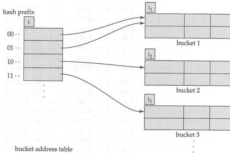
Figure 12.24 General extendable hash structure.
