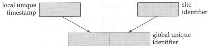
Figure 22.2 Generation of unique timestamps.
