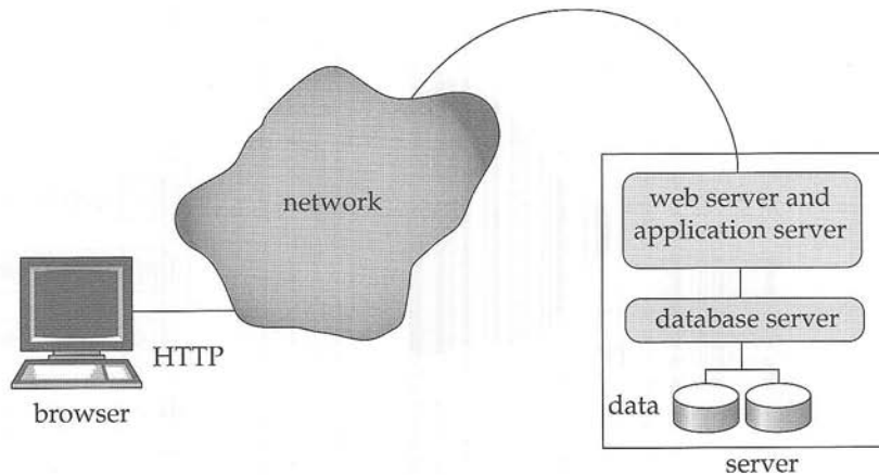
Figure 8.5 Two-layer Web architecture.
