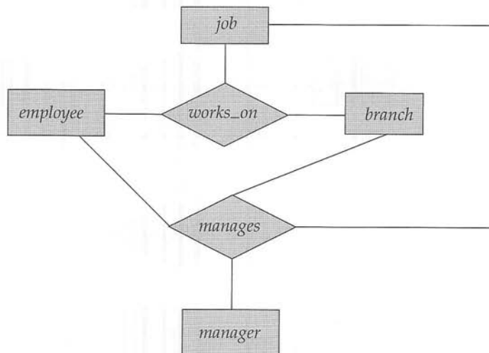
Figure 6.21 E-R diagram with redundant relationships.
