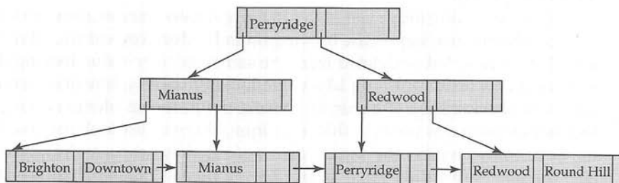
Figure 16.21 B^+ -tree for account file with n = 3 .
