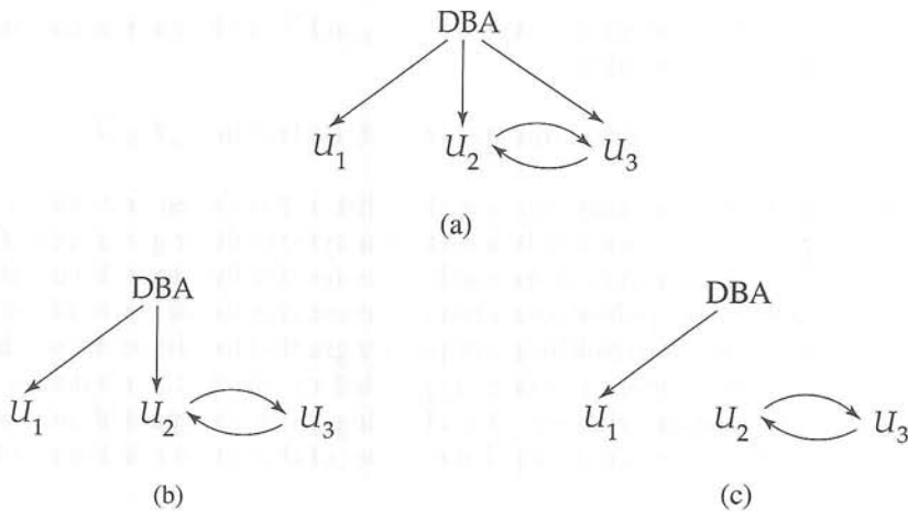
Figure 8.12 Attempt to defeat authorization revocation.
