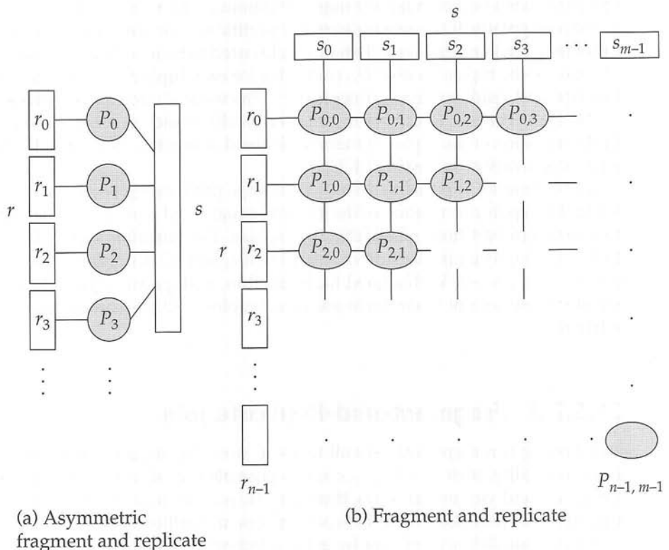
Figure 21.3 Fragment-and-replicate schemes.
