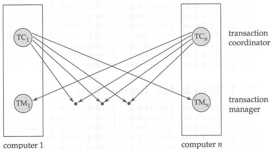
Figure 22.1 System architecture.
