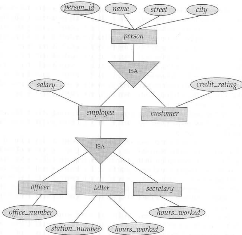
Figure 6.20 Specialization and generalization.
