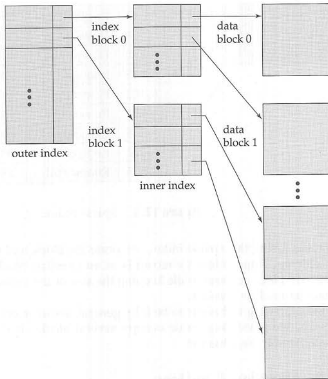
Figure 12.4 Two-level sparse index.
