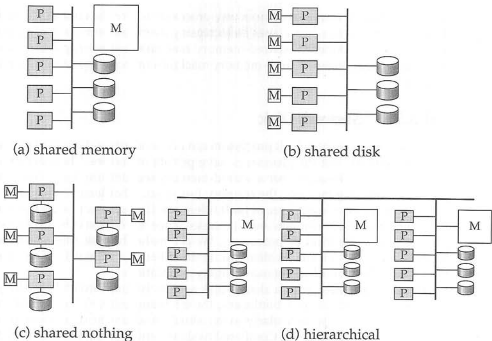
Figure 20.8 Parallel database architectures.
