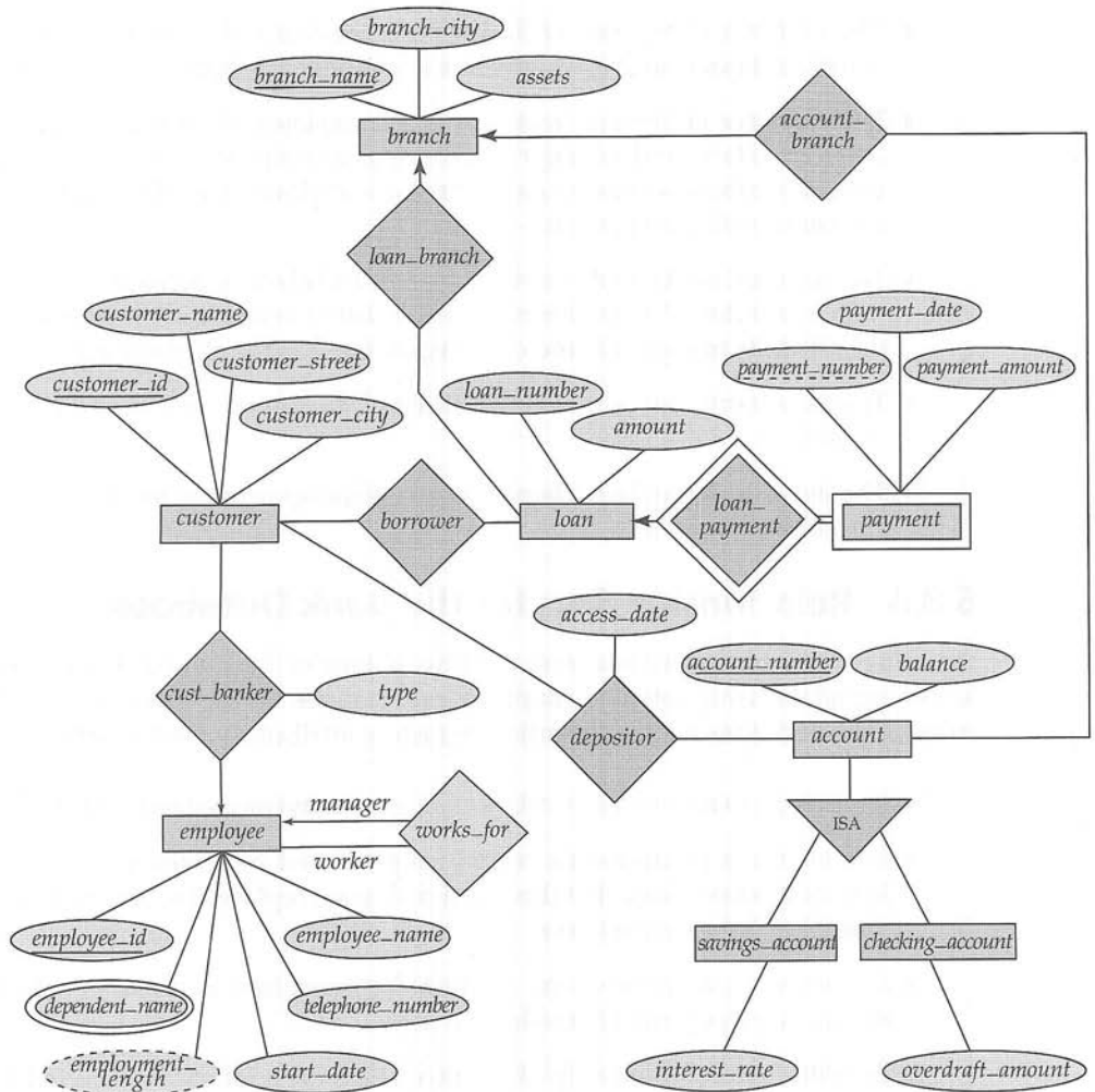
Figure 6.25 E-R diagram for a banking enterprise.
