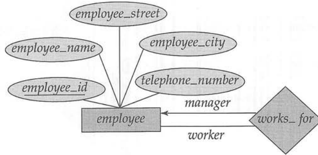
Figure 6.11 E-R diagram with role indicators.
