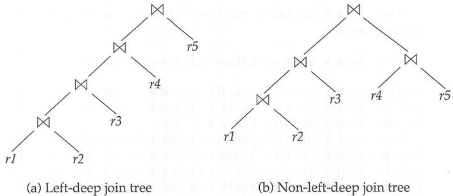
Figure 14.7 Left-deep join trees.
