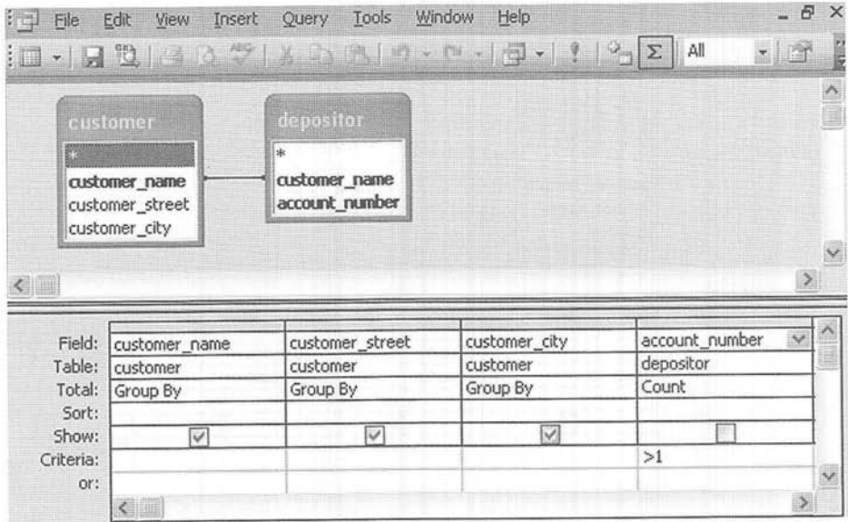
Figure 5.4 An aggregation query in Microsoft Access QBE.
