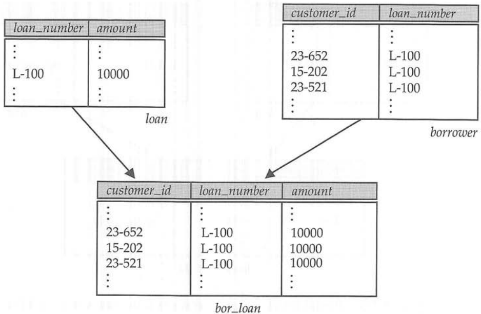
Figure 7.2 Partial list of tuples in relations loan , borrower , and bor_loan .
