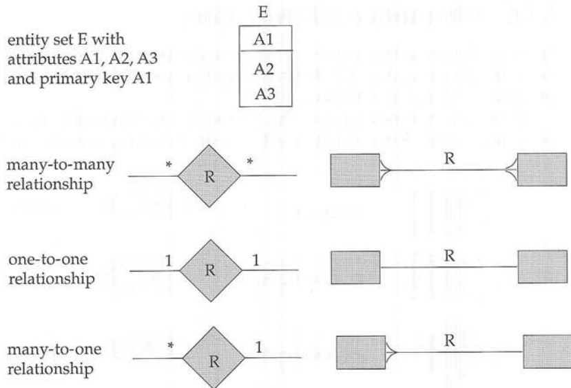
Figure 6.24 Alternative E-R notations.
