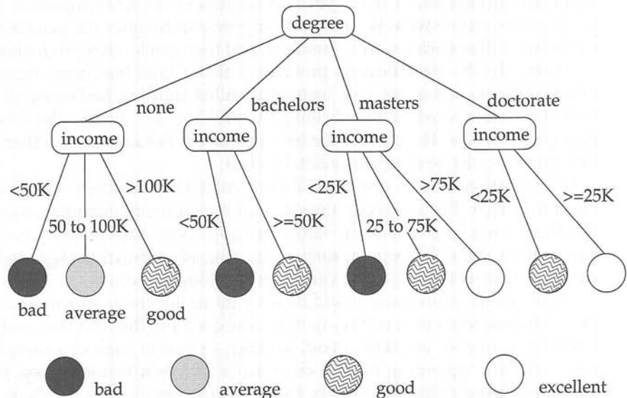
Figure 18.8 Classification tree.
