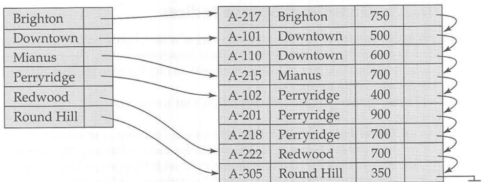
Figure 12.2 Dense index.
