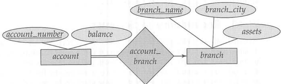
Figure 6.27 E-R diagram.
