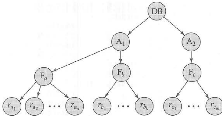
Figure 16.16 Granularity hierarchy.
