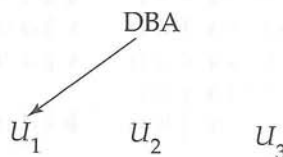
Figure 8.13 Authorization graph.
