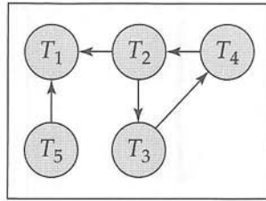
Figure 22.4 Global wait-for graph for Figure 22.3.
