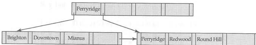
Figure 12.9 B + -tree for account file with n = 5 .
