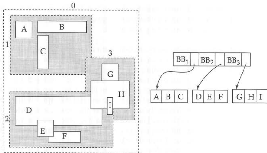
Figure 24.6 An R-tree.
