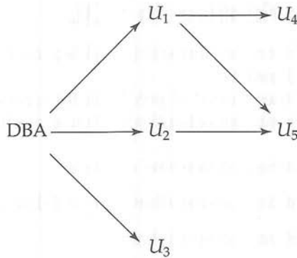
Figure 8.11 Authorization-grant graph.
