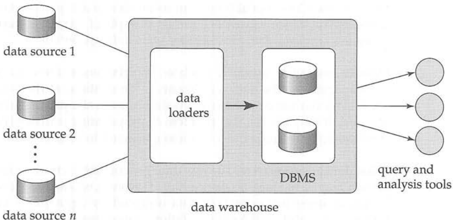
Figure 18.6 Data-warehouse architecture.
