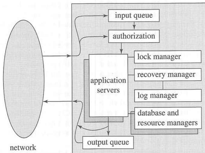
Figure 25.2 TP-monitor components.
