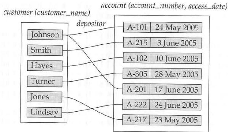
Figure 6.18 Access_date as attribute of the account entity set.
