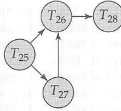
Figure 16.18 Wait-for graph with no cycle.
