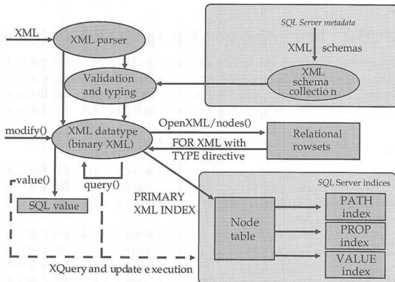
Figure 29.6 Architectural overview of the native XML support in SQL Server.
