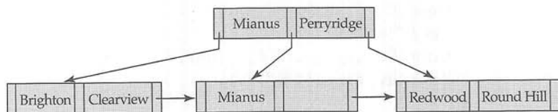
Figure 12.15 Deletion of “Perryridge” from the B + -tree of Figure 12.14.
