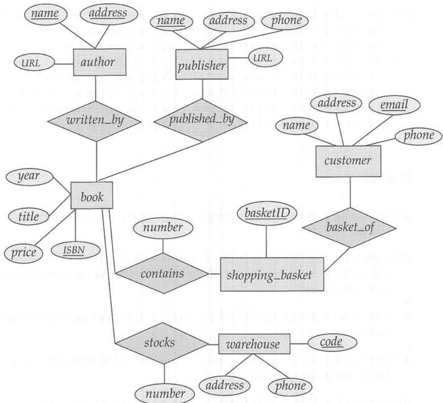
Figure 6.31 E-R diagram for Exercise 6.21.
