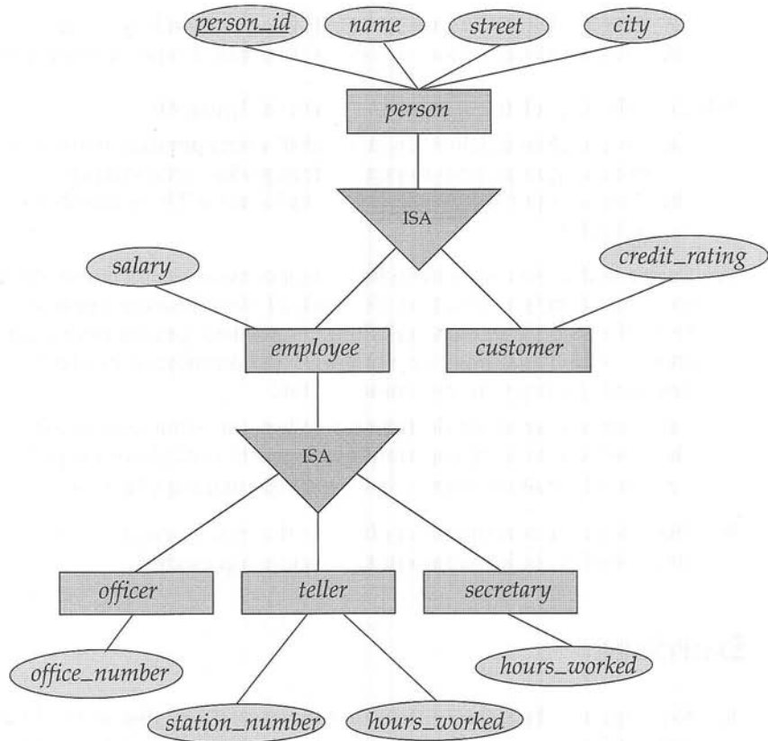
Figure 9.7 Specialization and generalization.
