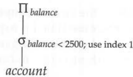
Figure 13.2 A query-evaluation plan.
