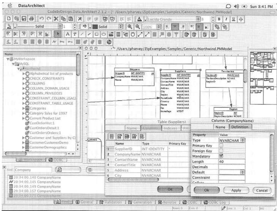
Figure 26.2 Data Architect: A multiplatform database design GUI.
