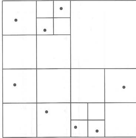
Figure 24.5 Division of space by a quadtree.
