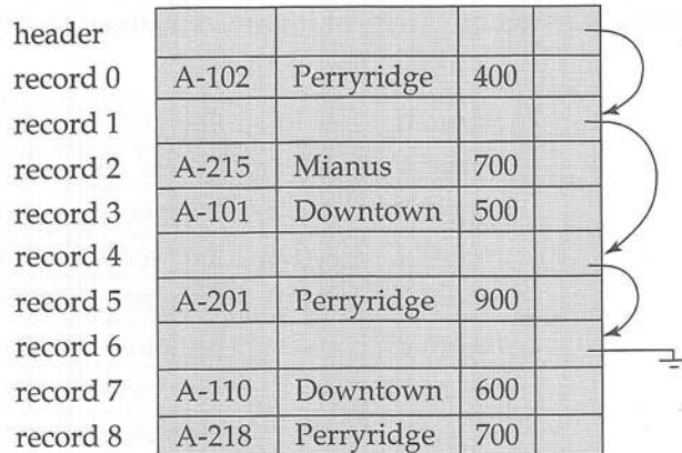
Figure 11.8 File of Figure 11.5, with free list after deletion of records 1, 4, and 6.
