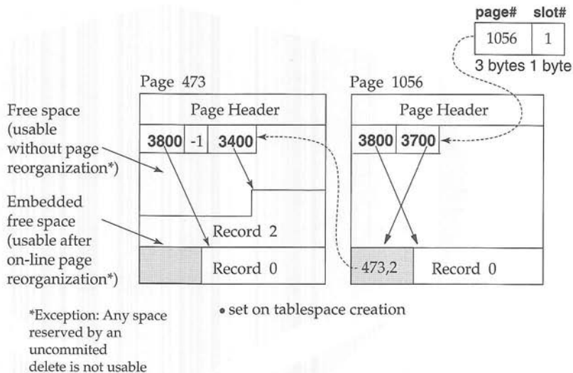
Figure 28.8 Data page and record layout in DB2.
