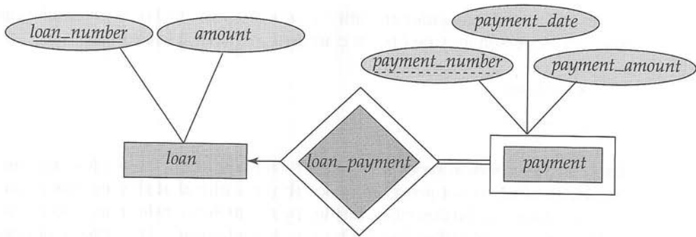
Figure 6.19 E-R diagram with a weak entity set.
