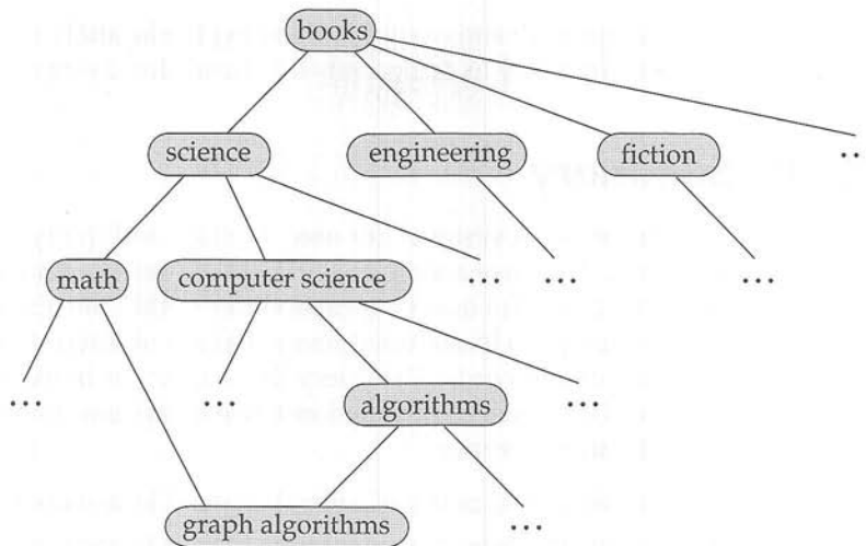
Figure 19.2 A classification DAG for a library information-retrieval system.
