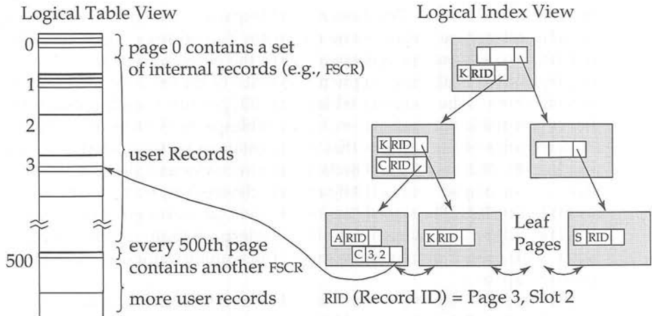
Figure 28.7 Logical view of tables and indices in DB2.
