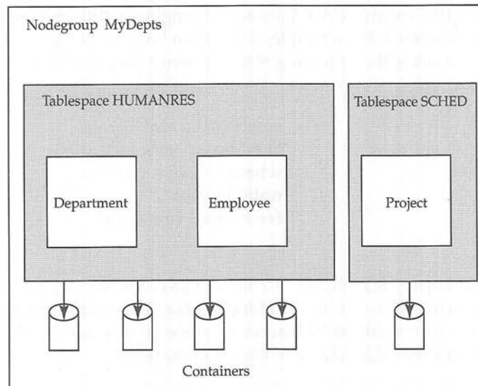
Figure 28.6 Tablespaces and containers in DB2.
