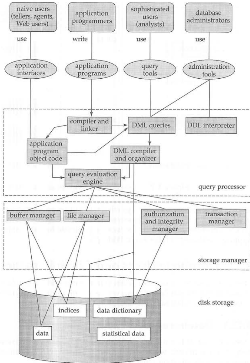
Figure 1.6 System structure.
