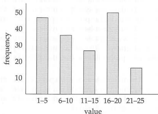
Figure 21.1 Example of histogram.
