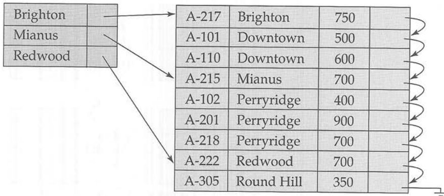
Figure 12.3 Sparse index.
