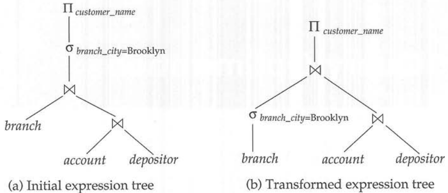
Figure 14.1 Equivalent expressions.
