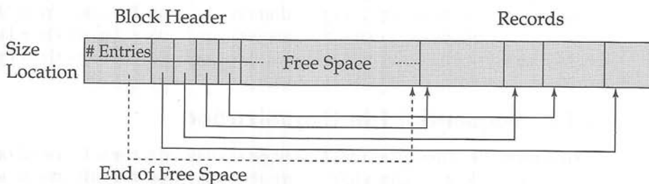
Figure 11.9 Slotted-page structure.
