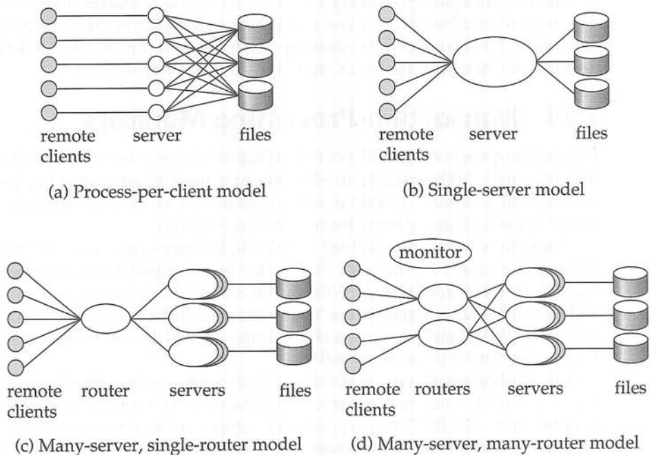
Figure 25.1 TP-monitor architectures.
